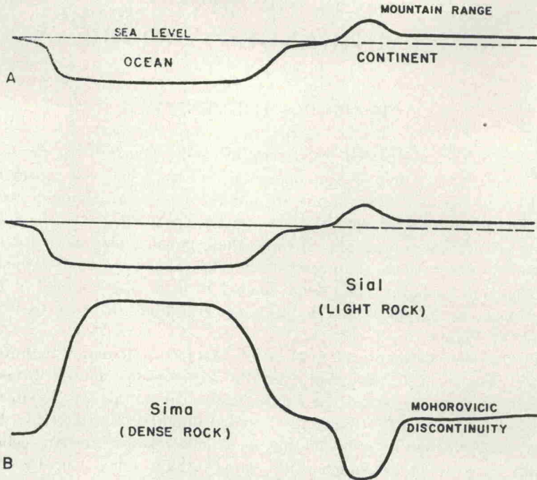
Fig. 1. Profiles through the Earth's crust
