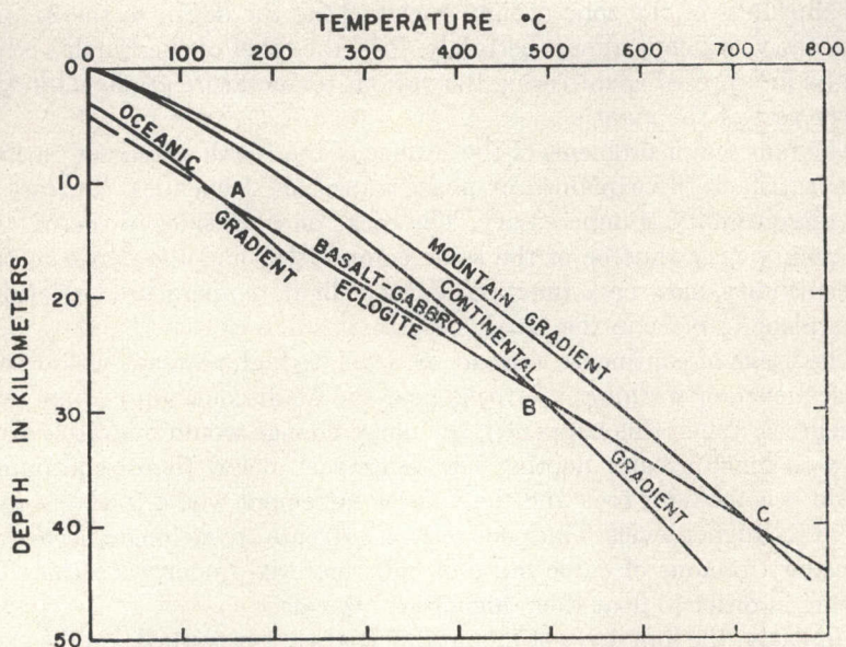
FIG. 2. Postulated temperature gradients under mountain ranges, continental areas, and oceanic regions.
